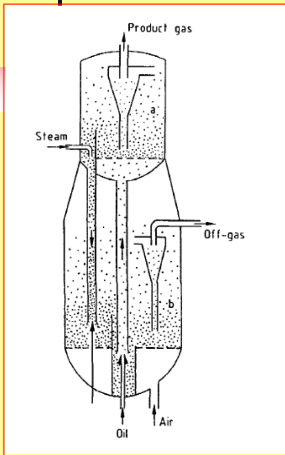
FCC (Kellogg-Orthoflow system) a - reaktor b - regenerator
