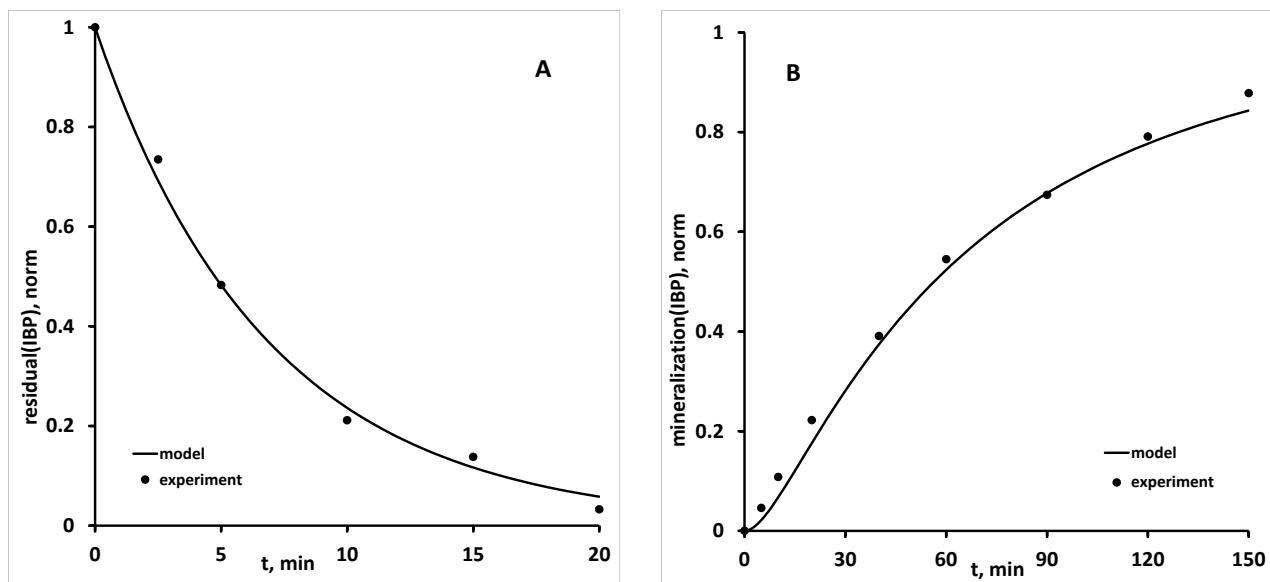
Figure 14 Graphical representation of the model simulation of photodegradation of IBP by UV-A/TiO 2 process at 1.2 g L -1 concentration of TiO 2 P25 A) conversion, B) mineralization
