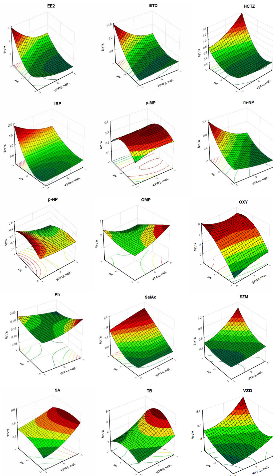
Figure 19 3D surface and contour diagrams showing the effect of mutual interactions between initial pH values ( X_1 ) and TiO_2 P25 loading ( X_2 ) on the response, adsorption constant ( K, L g^{-1} ), for organic compounds (Table S3)
