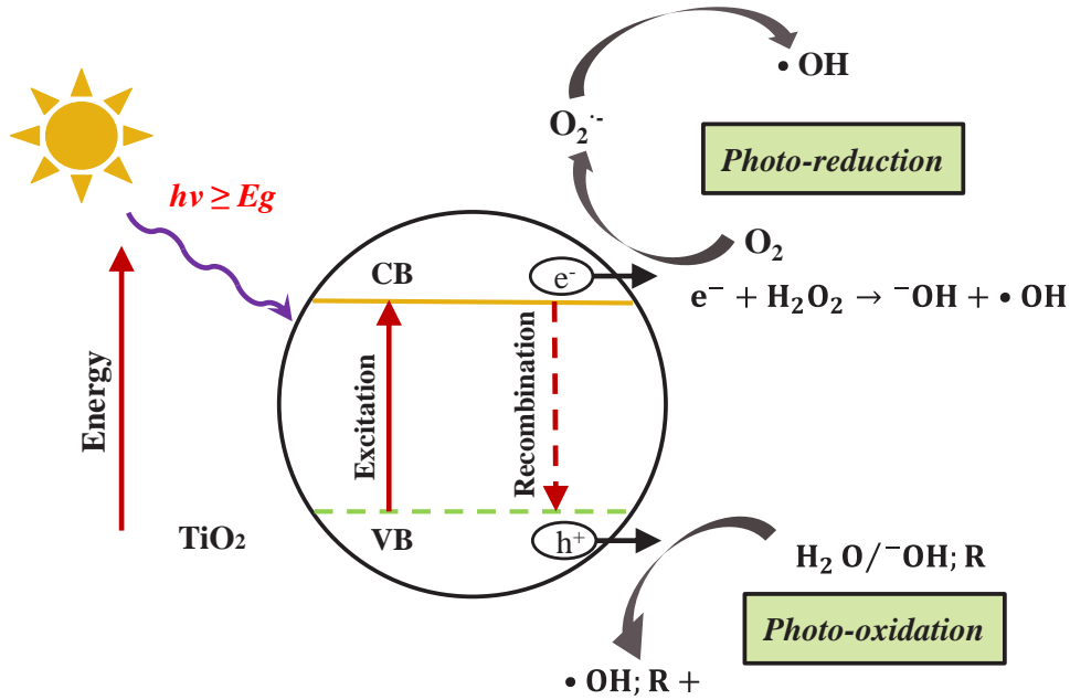
Figure 2 Simplified mechanism of the photocatalytic process
