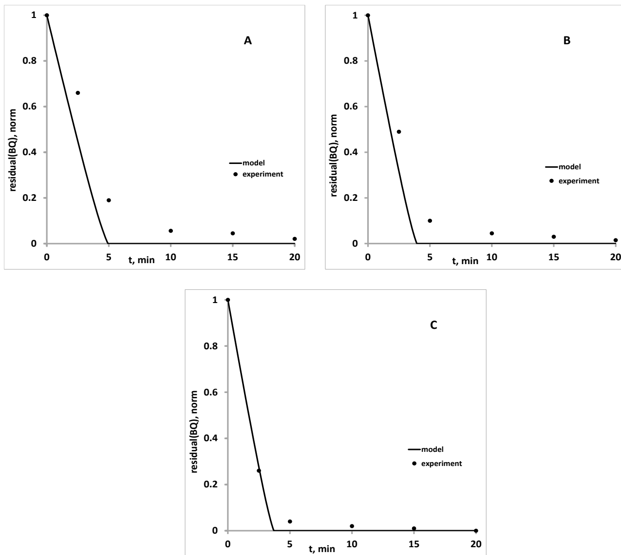
Figure 13 Graphical representation of the experimental and simulation results of photodegradation of BQ at different catalyst concentration of TiO 2 P25 by UV-A/TiO 2 processes: A) 0.4 g L -1 , B) 0.8 g L -1 , C) 1.2 g L -1
