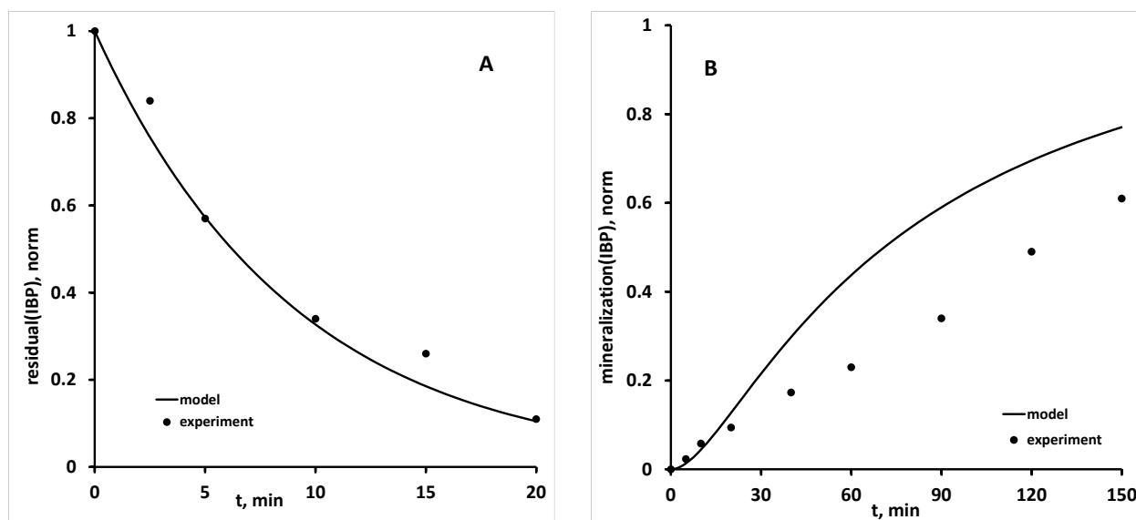
Figure 15 Graphical representation of the model simulation of photodegradation of IBP by UV-A/TiO 2 process at 0.4 g L -1 concentration of TiO 2 P25 A) conversion, B) mineralization
