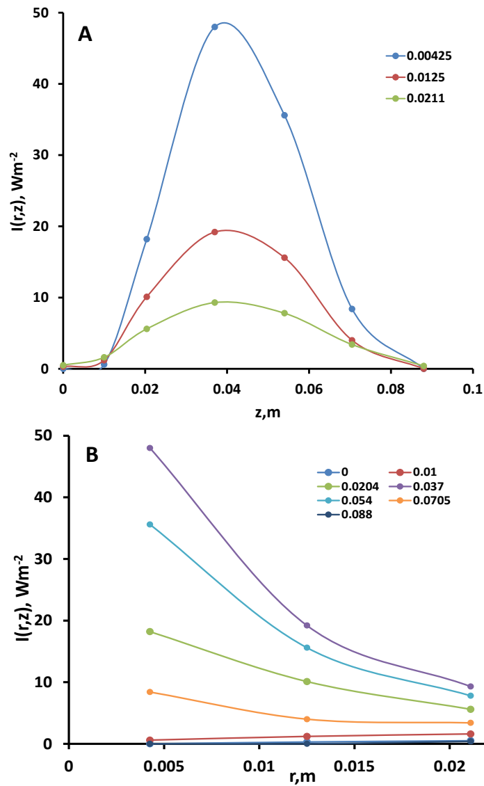
Figure 8 Irradiation intensity in photocatalytic reactor at the inner radius of the reactor annulus as a function of A) axial and B) radial measurement of irradiation of z and r points.
