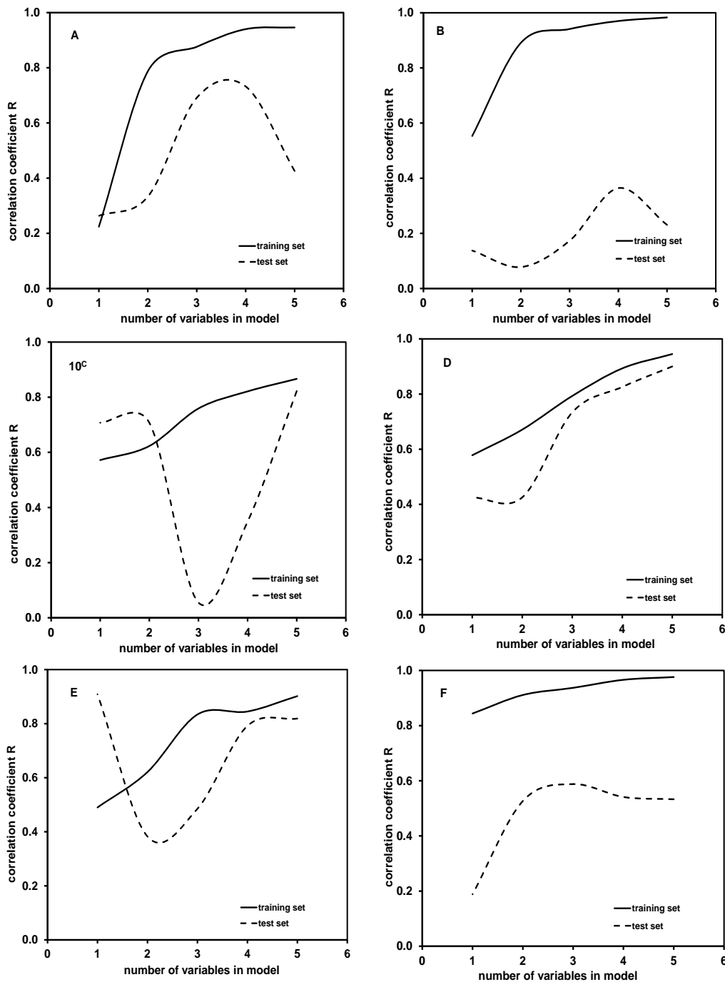
Figure 20 Comparison of correlation coefficients obtained for training and test set by 1 – 5 variable models for modelling of A, B, C, D, E and F coefficients of the RSM models
