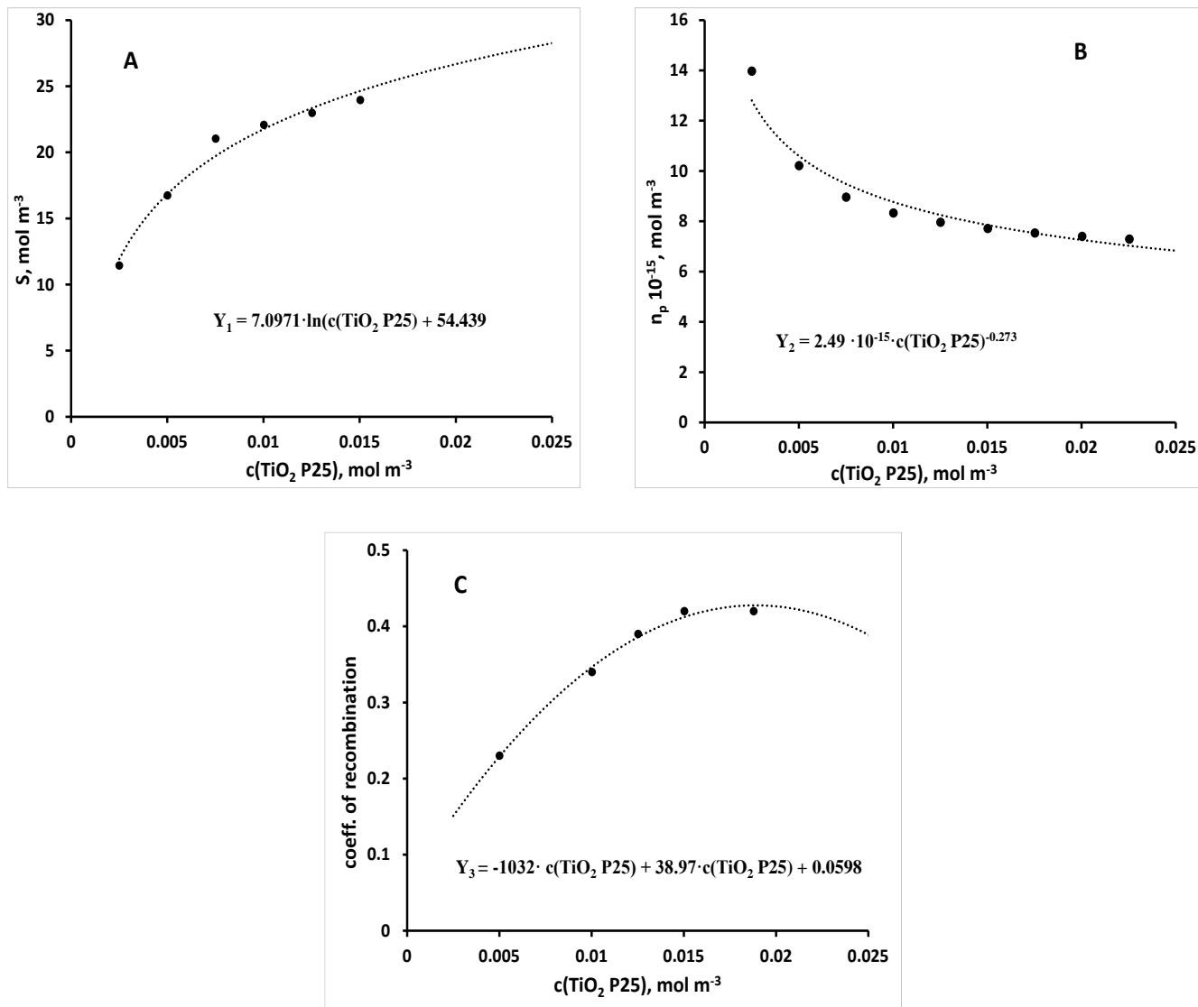
Figure 11 Mathematically dependence A) available adsorption sites on the catalyst and concentration of TiO 2 P25, B) average photon density in the volume of the reactor and concentration of TiO 2 P25, C) coefficient of recombination and concentration of TiO 2 P25
