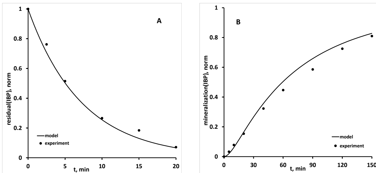
Figure 16 Graphical representation of the model simulation of photodegradation of IBP by UV-A/TiO 2 process at 0.8 g L -1 concentration of TiO 2 P25 A) conversion, B) mineralization
