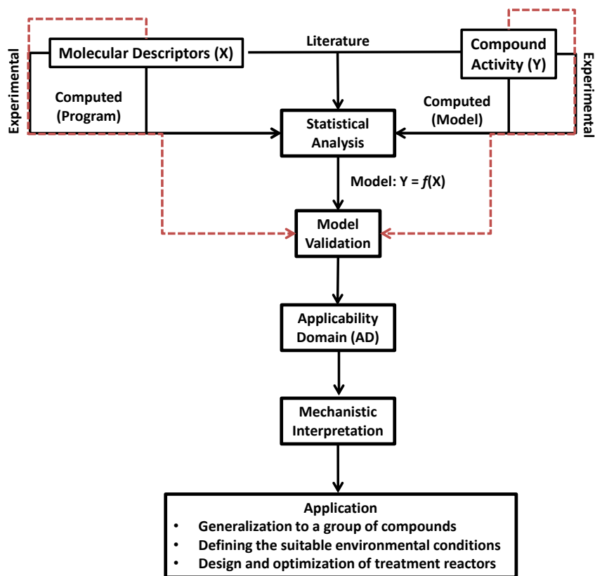
Figure 4 Simplified flow diagram for the development of a QSA/PR model [181]
