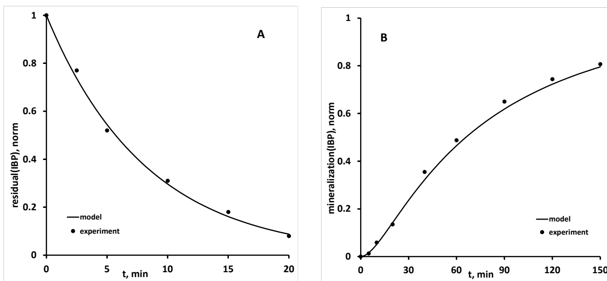
Figure 17 Graphical representation of the model simulation of photodegradation of IBP by UV-A/TiO 2 process at 2.0 g L -1 concentration of TiO 2 P25 A) conversion, B) mineralization
