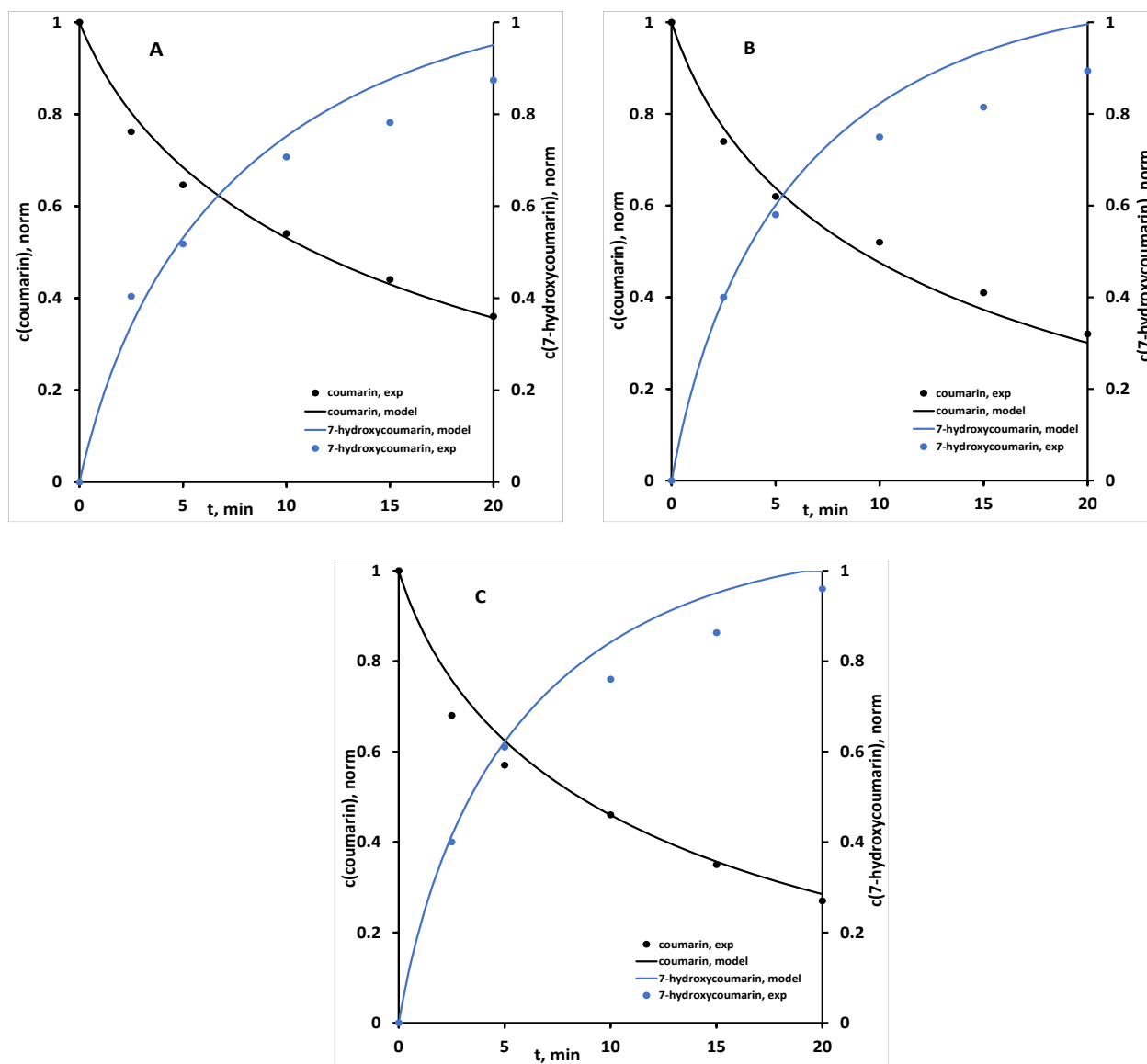
Figure 12 Graphical representation of the experimental and simulation results of photodegradation of coumarin and formation 7-hydroxycoumarin by UV-A/TiO 2 processes at different concentration of catalyst TiO 2 P25 A) 0.4 g L -1 , B) 0.8 g L -1 , C) 1.2 g L -1
