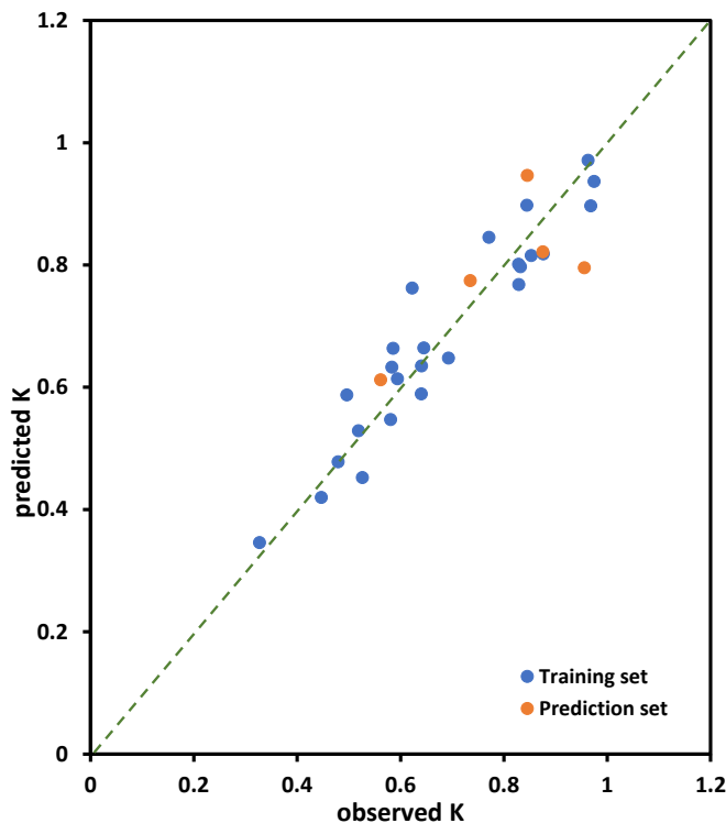
Figure 31 The observed vs. predicted values for K coefficient (in transformed \frac{1}{\sqrt{K+1}} form), for the entire set (30 compounds) calculated by 5 variable model
