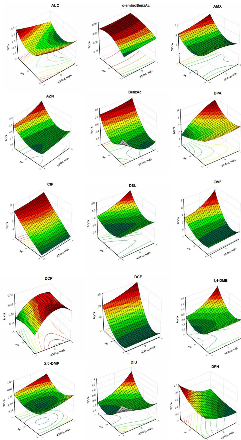
Figure 18 3D surface and contour diagrams showing the effect of mutual interactions between initial pH values ( X_1 ) and \text{TiO}_2 P25 loading ( X_2 ) on the response, adsorption constant ( K, \text{L g}^{-1} ), for organic compounds (Table S3)
